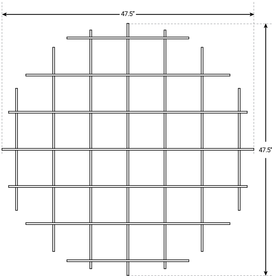
TOP VIEW
