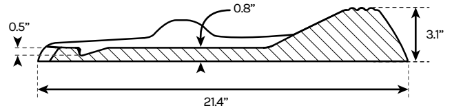
SIDE VIEW cross section [A]
